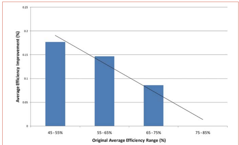
Figure 2. Efficiency improvements versus original efficiency in EBMUD.
