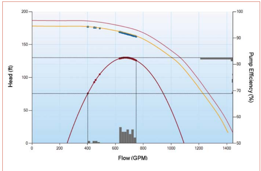
Figure 5. Real-time pump curve displayed on Dashboard display screen.
