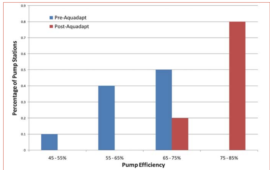
Figure 3. Efficiency improvement in pumps at EBMUD.
