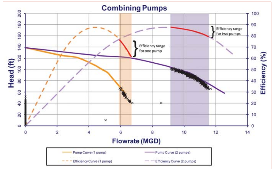
Figure 1. Pump curves for a single pump and two identical pumps running together.
