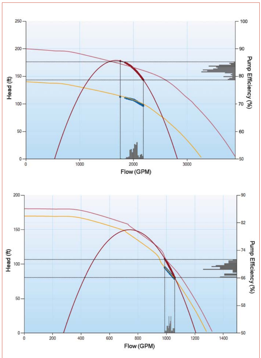
Figure 6. Two nominally identical pumps operating differently.
